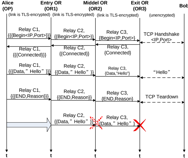
Fig. 9. Duplicate and Hold a Cell on Tor
