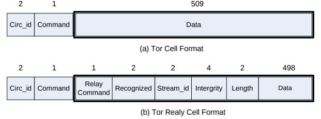
Fig. 2. Cell Format By Tor [8]
