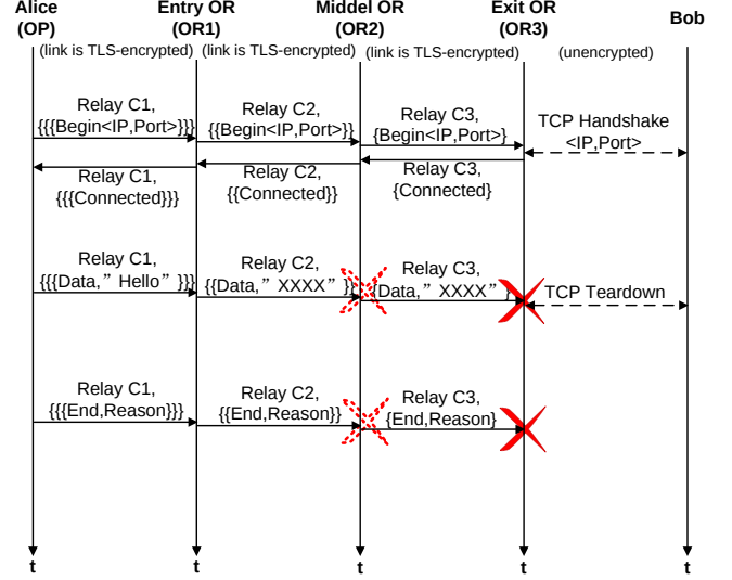
Fig. 6. Modify a Cell on Tor
