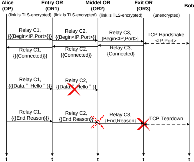
Fig. 8. Delete a Cell on Tor
